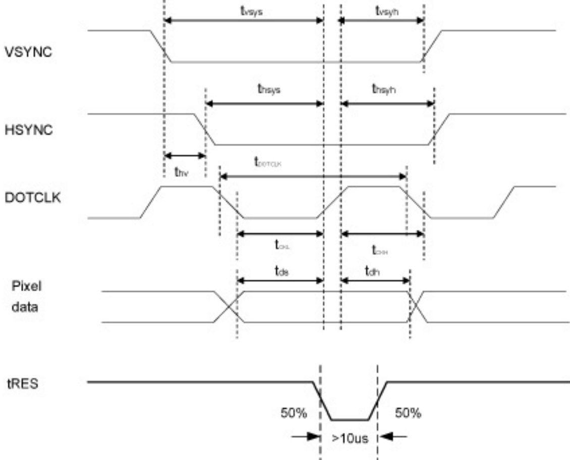
Figure 7. 1 Pixel Timing
