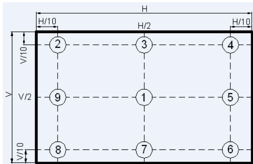
Figure 6 Measurement Locations
