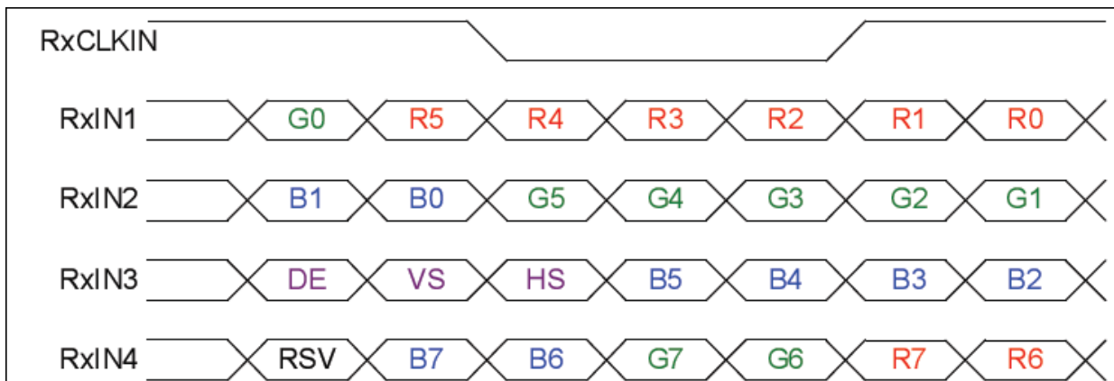
Figure 8 Timing Characteristics
