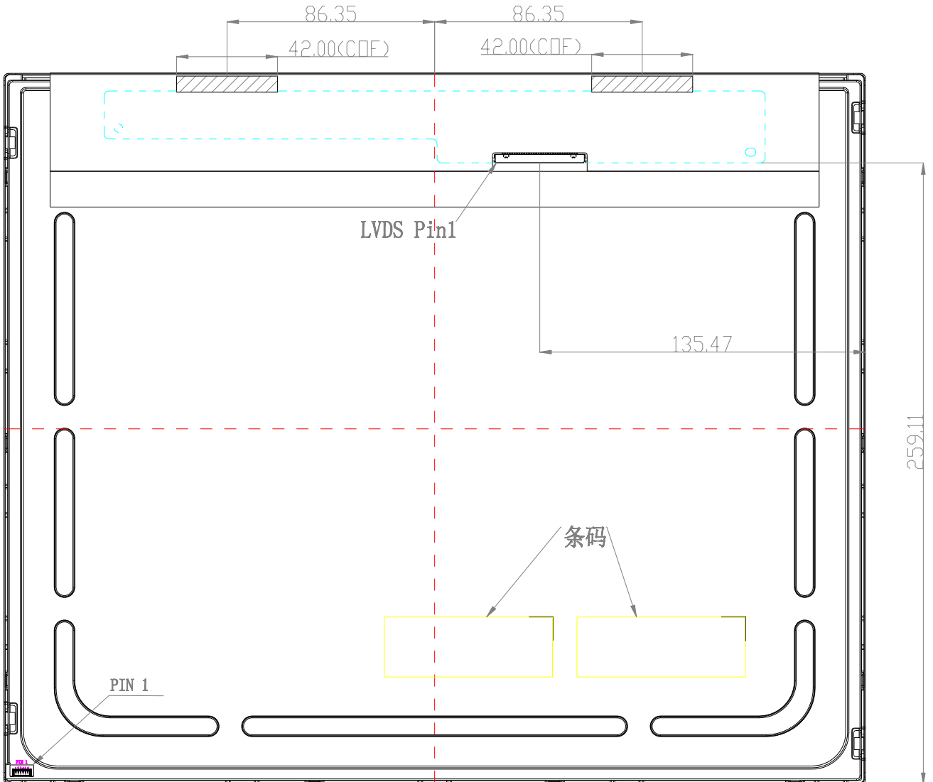
< Figure 5.TFT-LCD Module Outline Dimensions (Rear View) >
