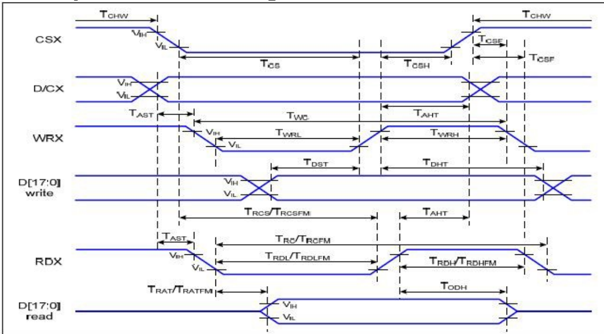
Figure 1 Parallel Interface Timing Characteristics (8080-Series MCU Interface)
