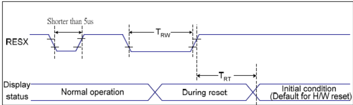
Figure 7 Reset Timing
