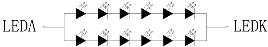
BL CIRCUIT DIAGRAM V_F=19.2V, I_F=40mA
